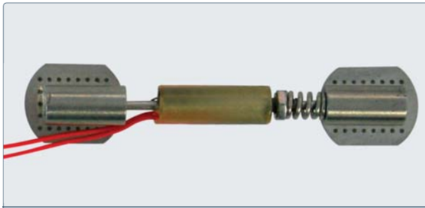
Vibrating Wire Spot Weldable Strain Gauge - Low Profile
